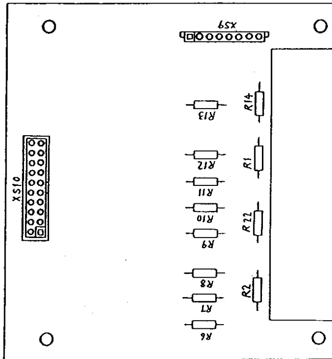
Fig.17 Component installing diagram of display board
