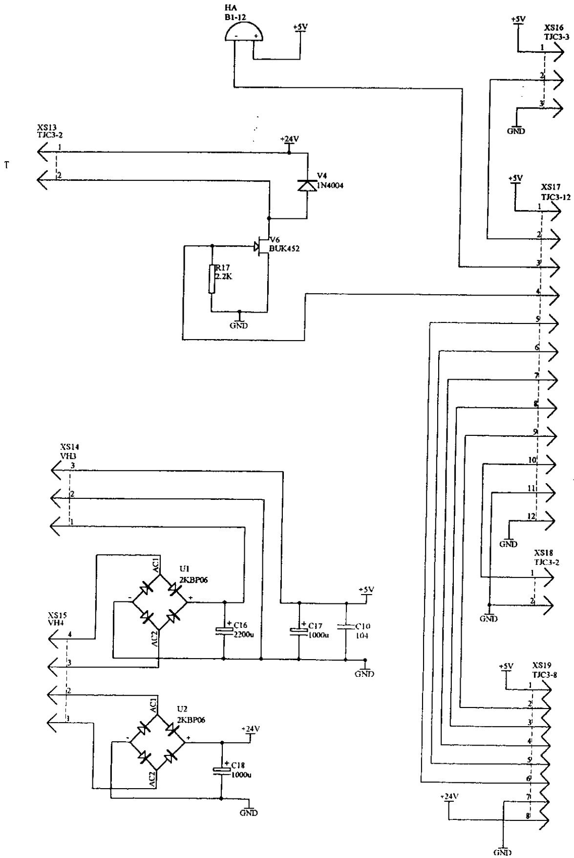
Fig.14 Electric circuit diagram of DC power supply board
